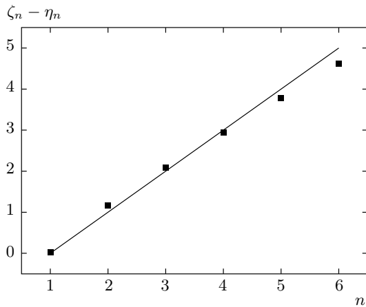
Fig. 10. The difference of the scaling exponents of moments for the integral passive scalar and for the passive scalar, \zeta_n - \eta_n , computed at \delta = 0.03125 in 2d . For comparison, the theoretical prediction n - 1 is drawn
