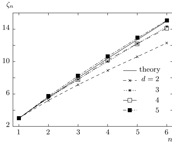
Fig. 8. Exponents of the moments \langle \Theta_\delta^n \rangle , for n = 1-6 and space dimensions d = 2-5 . For comparison, the theoretical curve \zeta_n = 2n - 1/2 + \sqrt{2n + 1/4} is plotted (solid line)
