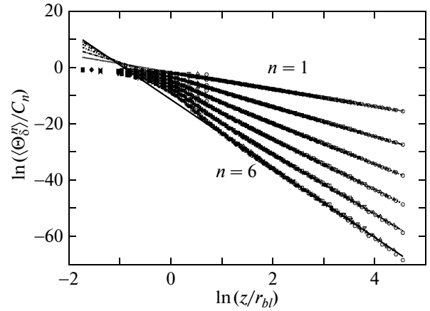
Fig. 6. Moments of \Theta_\delta in log-log coordinates, n = 1-6 . In the region z > r_{bl} , the results collapse onto single curves for three times \tau = 0.001, 0.002 , and 0.004 and four different values of the diffusion coefficient
