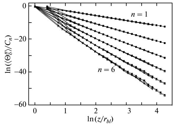
Fig. 7. Moments of \Theta_\delta in logarithmic coordinates, n = 1-6 . The results are obtained for two cases where the diffusion occurs everywhere and where it is switched off at z > 3 , and also for two different velocity fields: with two and four harmonics
