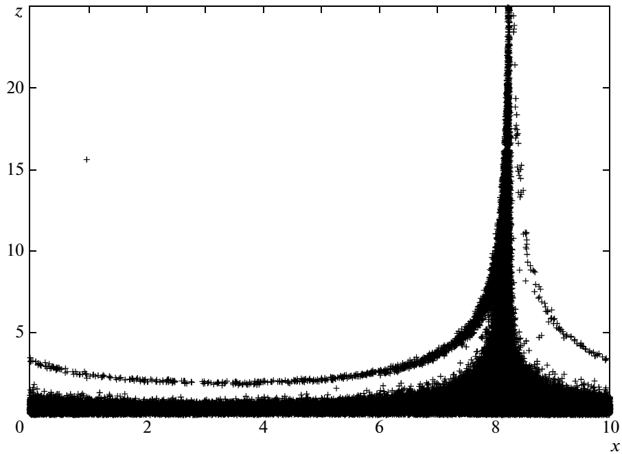
Fig. 2. An example of a passive scalar structure formed near the wall in a 2d random flow. Different particles are designated by small crosses
