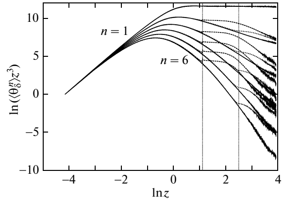
Fig. 4. Log-log plot of the moments \langle \theta_\delta^n \rangle z^3 , for \delta = 0.03125 and n = 1-6 . The graph reflects simulations where diffusion occurs everywhere, and is switched off at z = 3 or z = 12
