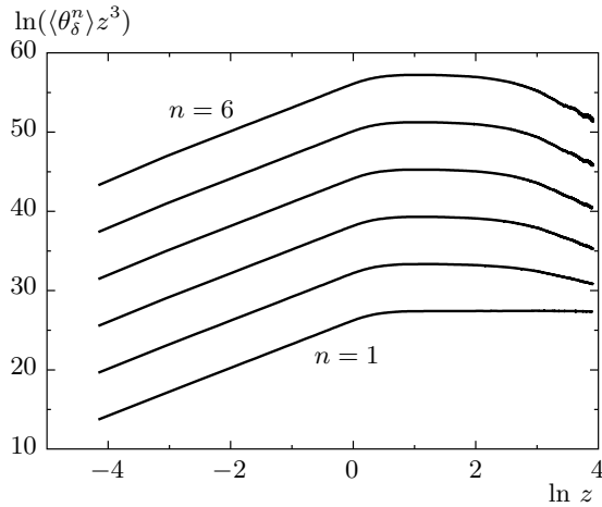
Fig. 5. Log-log plot of the moments \langle \theta_\delta^n \rangle times z^3 , for \delta = 0.03125 and n = 1-6 in the case where diffusion is substituted by a constant velocity carrying the particles away from the wall
