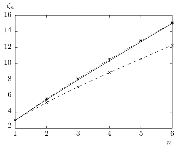
Fig. 9. Exponents of the moments \langle \Theta_\delta^n \rangle , for n = 1-6 and space dimension d = 2 for two different velocity fields: containing only the first harmonic (dashed line) and three (9th, 10th, and 11th) harmonics (dotted line). For comparison, the theoretical curve \zeta_n = 2n - 1/2 + \sqrt{2n + 1/4} is plotted (solid line)
