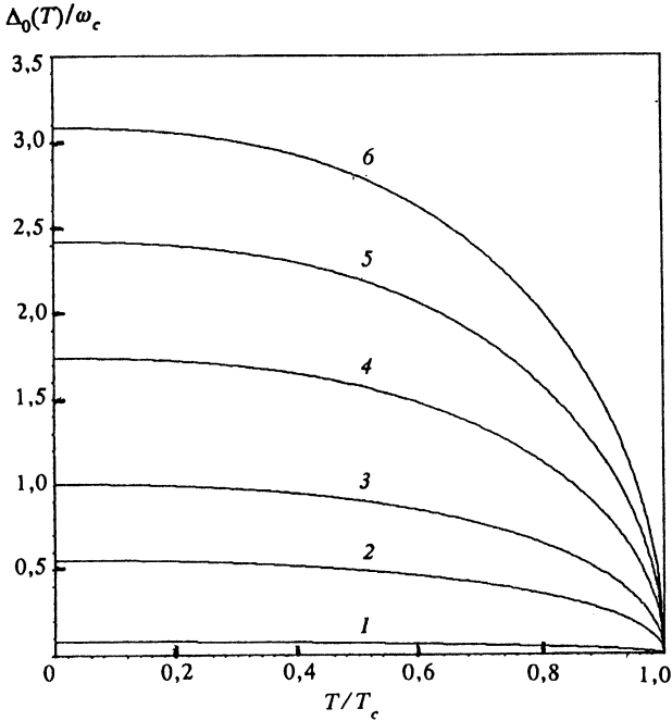
FIG. 2. Temperature dependence of \Delta_0(T) in the case of "odd" pairing for several values of the pairing coupling constant. Curve 1 corresponds to g=1.22 , curve 2 to 1.5, curve 3 to 2.0, curve 4 to 3.0, curve 5 to 4.0, and curve 6 to 5.0.
