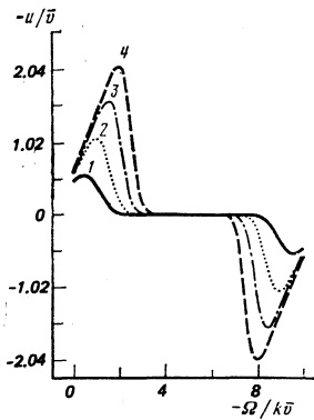
FIG. 3. Dependence of the drift velocity in a radiation field with rectangular spectrum of width \Delta = 10 k\bar{v} on the distance from the left edge of the spectrum to the center of the transition at different values of the parameter \bar{\kappa}_{\text{rect}} = 2|G|^2/\Delta (\Gamma_m + \nu_m) and on the ratio of the collision frequencies \nu_m/\nu_n . The maximum values of |u/\bar{v}| are reached at \bar{\kappa}_{\text{rect}} \gg \kappa_0 . 1) \nu_m/\nu_n = 10 , \kappa_0 = 0.08 ; 2) \nu_m/\nu_n = 10^2 , \kappa_0 = 0.03 ; 3) \nu_m/\nu_n = 10^3 , \kappa_0 = 0.03 ; 4) \nu_m/\nu_n = 10^4 , \kappa_0 = 0.02 .
