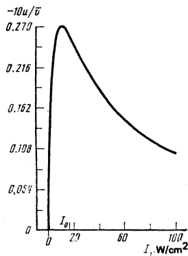
FIG. 1. Dependence of the drift velocity on the radiation intensity I with a broad Gaussian spectrum, \Omega = \beta = 10 k\bar{v} ; \nu_m/\nu_n = 10 ; I [W/cm^2] \approx 3.5 \kappa_G(\Omega) .
